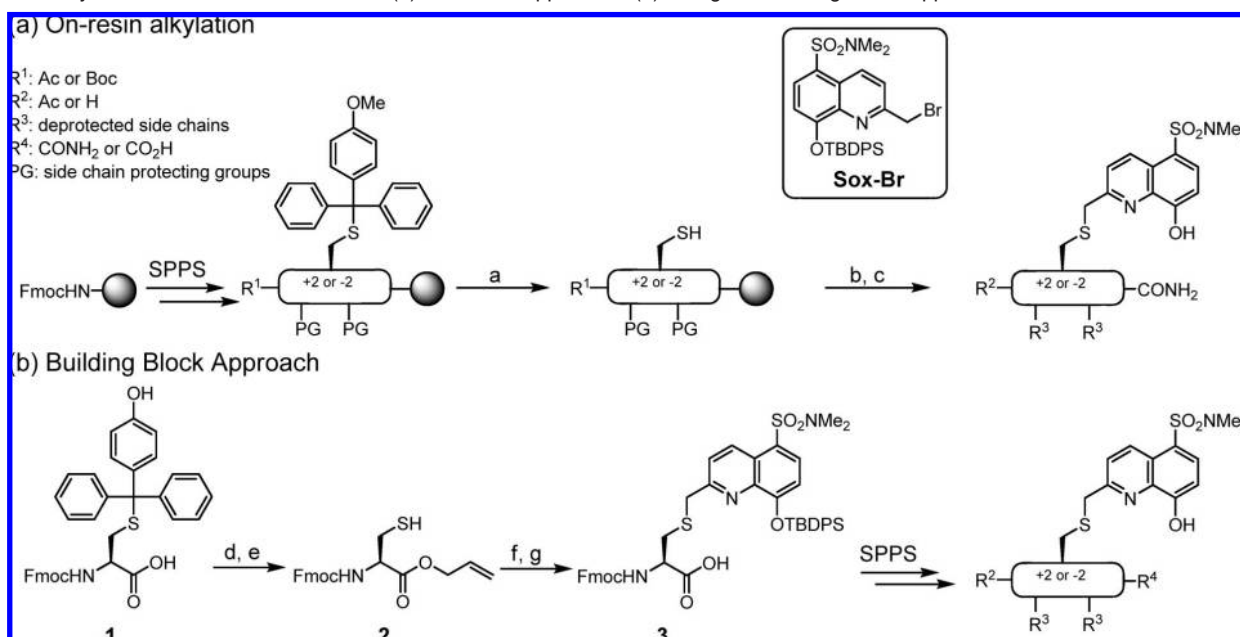
Scheme 1. Synthesis of RDF Chemosensors (a) on Solid Support and (b) Using the Building Block Approach a
